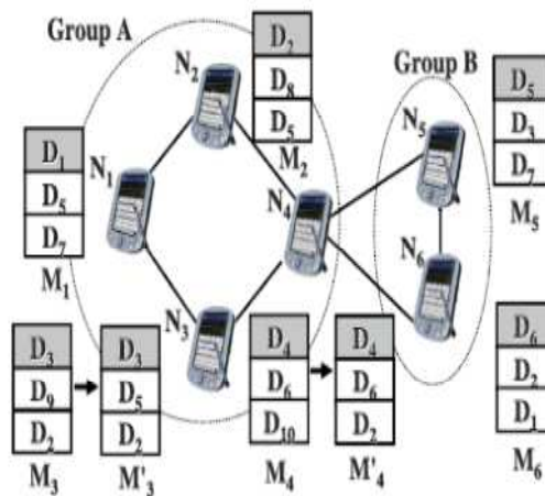
FIG. 1: SELFISH REPLICA ALLOCATION
