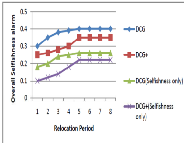
FIG. 3: RELOCATION PERIOD VS. OVERALL SELFISHNESS ALARM
